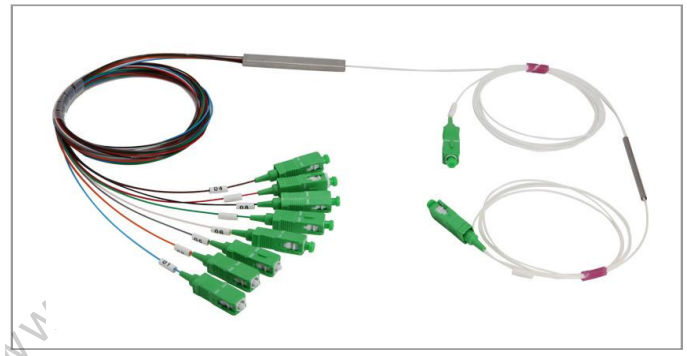
FBT+PLC MIX Optical Splitter
